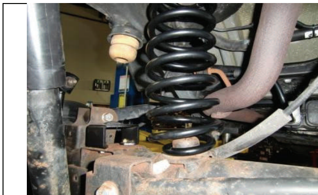
Install new coil springs and OE isolators and raise axle.
