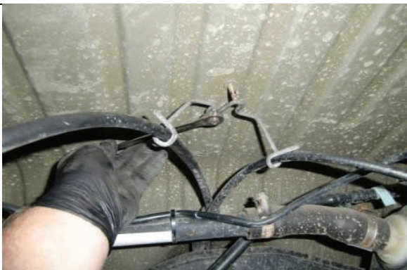
At the rear, remove center brake line nuts under body.
