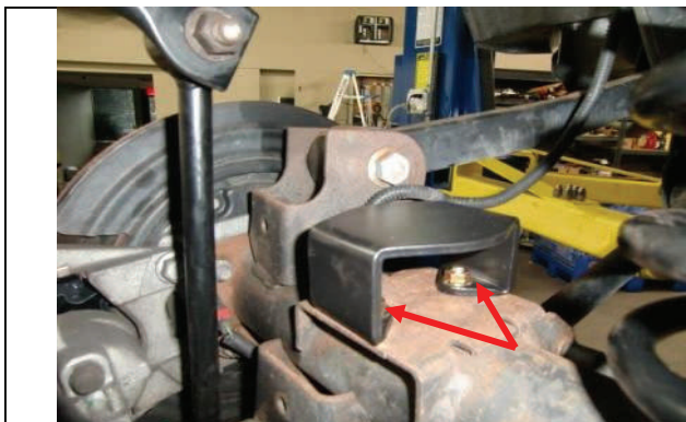
Install rear bump stop extensions with provided hardware.
