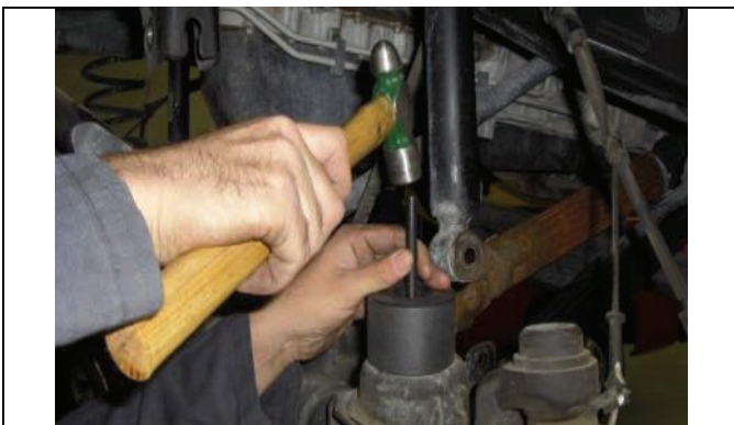
Center, mark and drill 11/32 hole for self tapping bolt.
