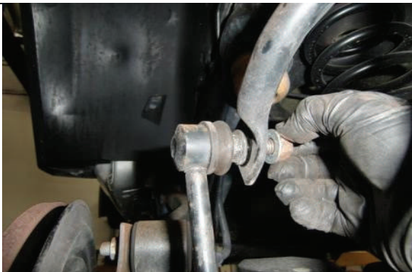
Disconnect and remove rear swaybar endlinks
