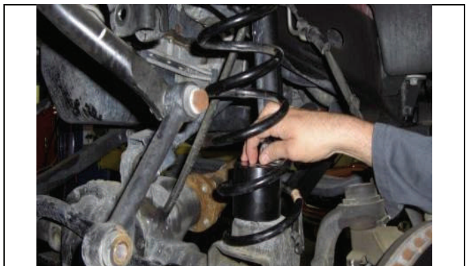
Install new springs/bumpstops extensions simultaneously.
