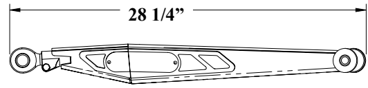
Rear Lower Control Arm 90-3802 drvr 90-3796 pass
