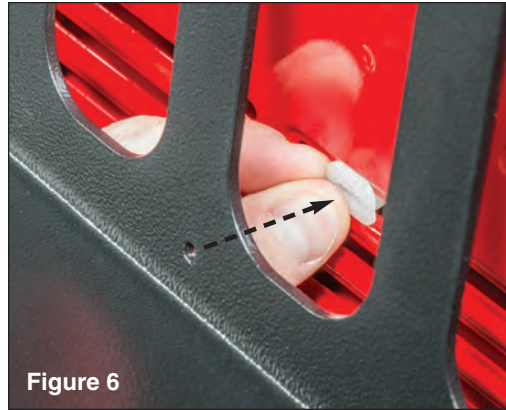
Figure 6 Insert the 4 Philips head screws and washers through the holes in the cargo shelf and align the plastic retaining clips accordingly; the clips will slide side to side in the tailgate vents.
