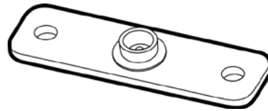
Snap Bracket Part # 507.83 One per side
