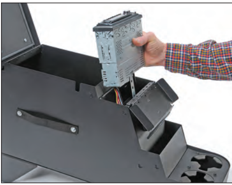
FIGURE 4. If you are not installing a radio please skip to step 6. Insert stereo assembly with attached wiring and stereo strap through the din slot. Fasten the other end of the stereo support strap at the 3/16" hole using a #10-32x1/2" bolt with 3/16" washer and secure with a #10-32 locknut. Connect all wires to the stereo according to your stereo owner's manual. Stereo wiring extensions may need to be fashioned or purchased separately.
