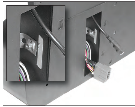
FIGURE 5. The metal stereo strap fastens to console wall as shown. If your stereo receiver features a rear auxiliary input, a rectangular opening is provided to allow the cord to pass through the inside of the main compartment.
