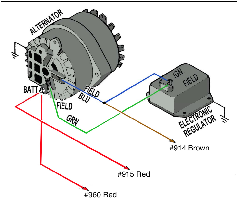
Diagram 11 Mopar Alternator
