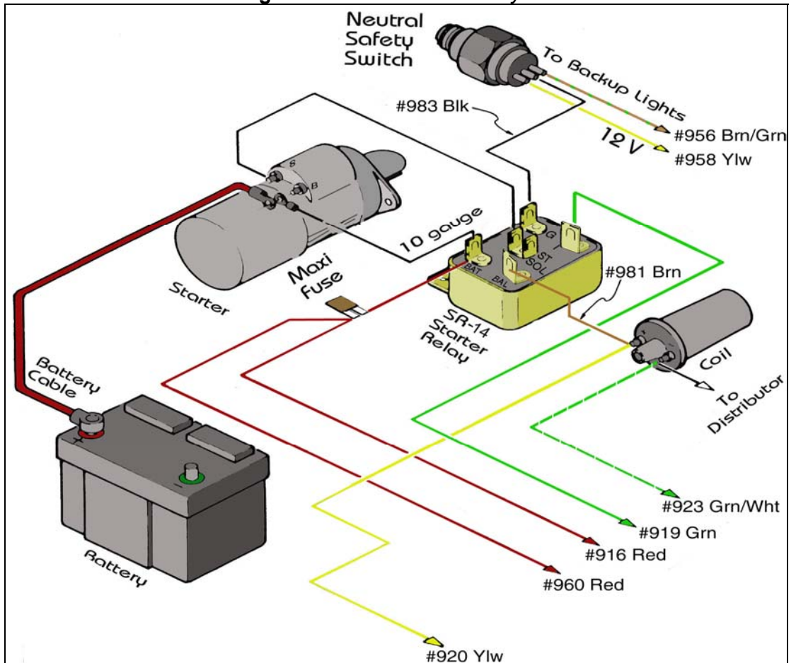
Diagram 14 Mopar Start/Run System
