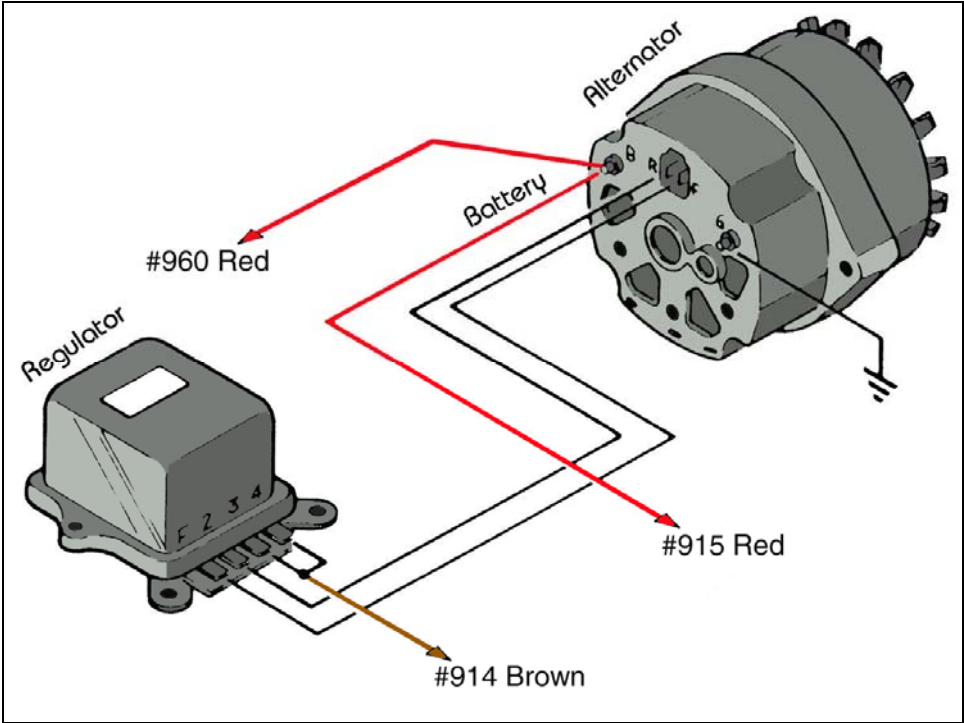
Diagram 10 Delco Alternator
