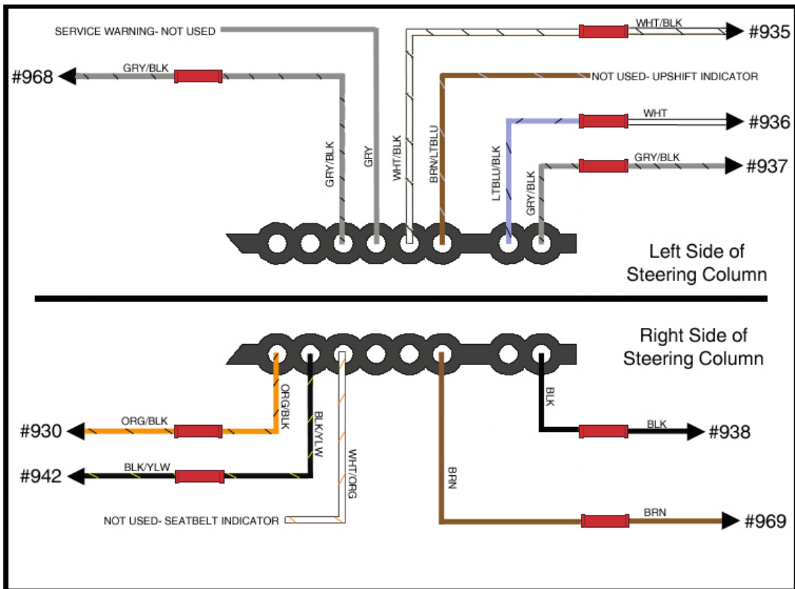
Diagram 1 Indicator Light Circuit Board Connectors
