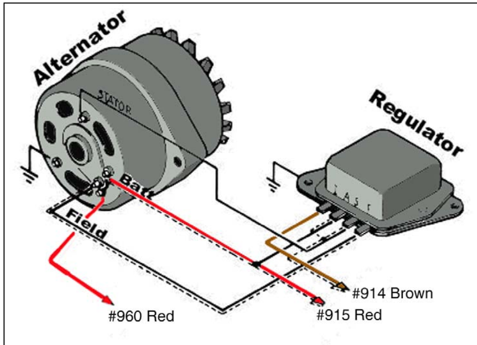
Diagram 12 Motorcraft Alternator
