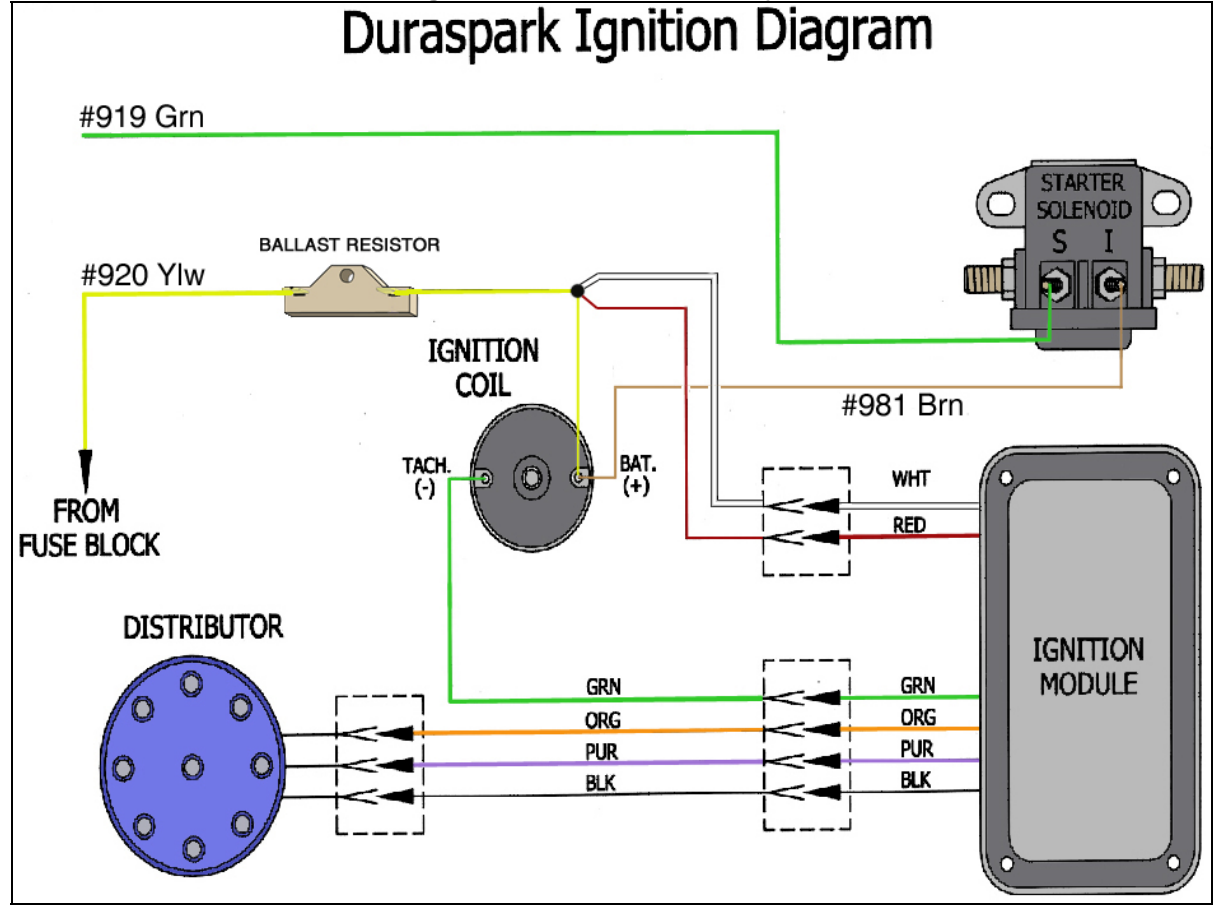
Diagram 16 Duraspark Ignition System
