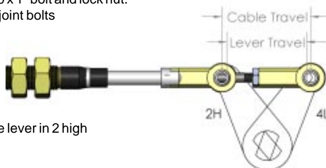
2007-2011 JK NP241 t-case shifter adjustment
