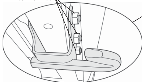
View from under bumper
