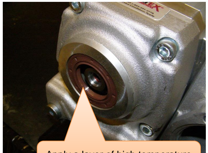
Apply a layer of high temperature lubrication grease (All around)
