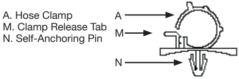
(Fig. 3) Leader Hose Bracket
