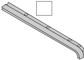
Windshield Retainer - Left, Qty - 1, Part Number 225.43
