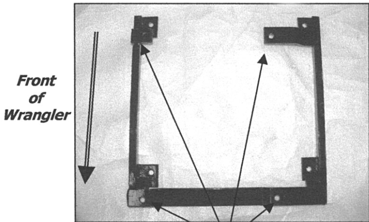
Seat Riser Attachment Holes
