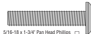
5/16-18 x 1-3/4" Pan Head Phillips Screw, Qty - 8, Part Number 387.91
