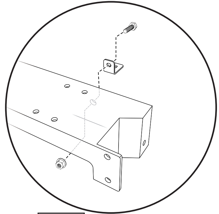
M8 Nylon Lock Nut Part #470.06 Qty. 1
