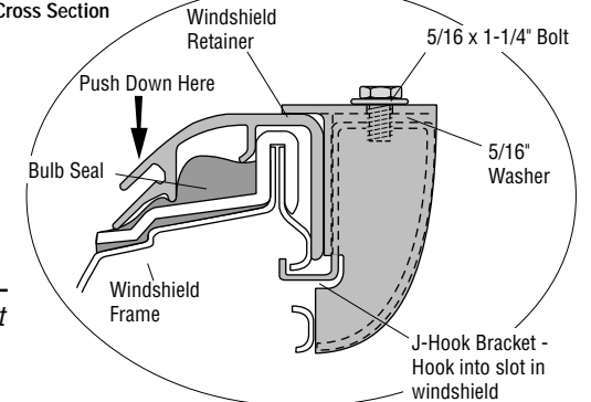
Windshield Retainer Cross Section
