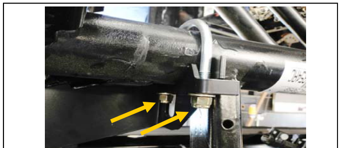
12. Install the u-bolt over the axle and into the bracket. Using the hardware provided torque down to 22 ft. lbs.
