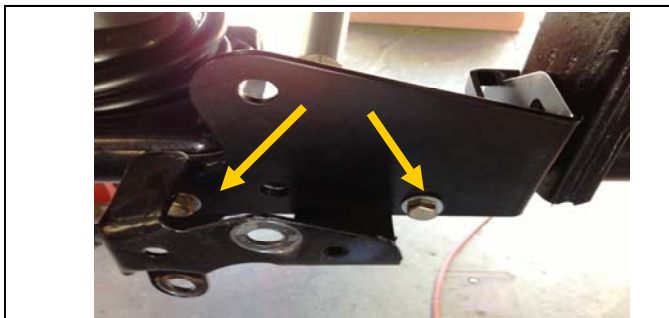
9. Install the passenger side front axle bracket to the inside of the pocket. Leave the hardware loose.
