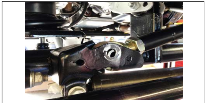
8. Remove the track bar from the axle side.
