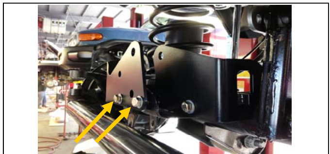
10. Install the passenger side front axle bracket to the outside of the pocket.
