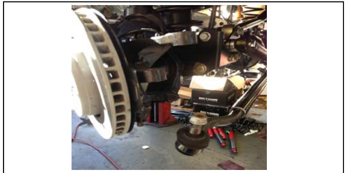
6. Remove the tie rod from the passenger side.
