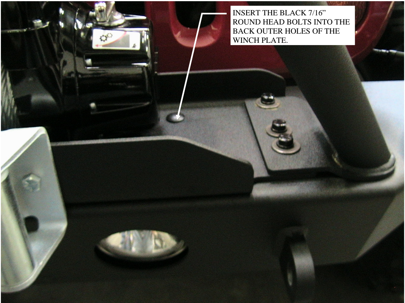
Figure 1: Winch Plate bolts locations
