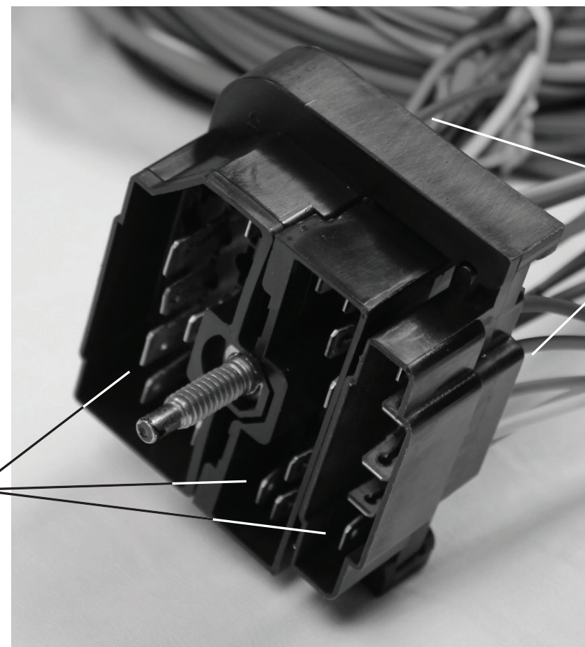
assembly, ready to bolt onto firewall bulkhead
