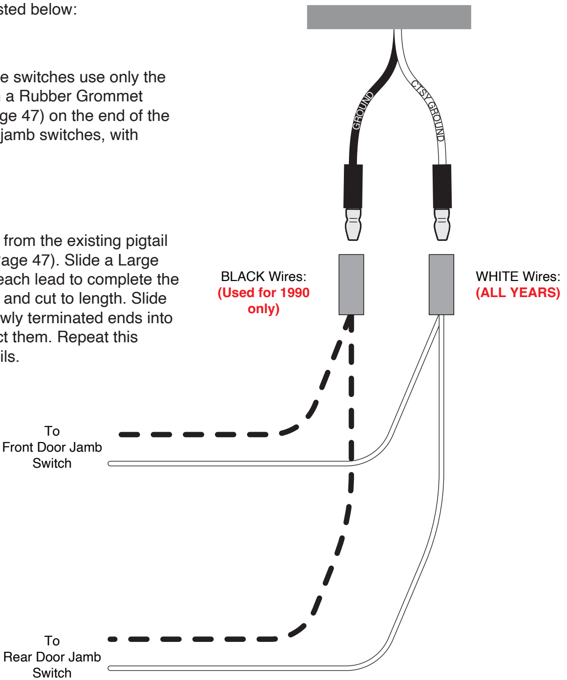
Door Jamb Switch Connections from Dash Harness (LH Connections Shown, RH Connections are identical)
