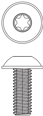
Screw, M8 X 20 mm Part #573.09 Qty. 2 (T40)
