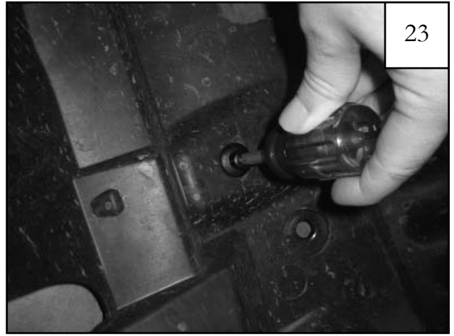
Using a Phillips screwdriver, reassemble inner structure and splash shield by installing supplied Plastic Phillips Head Tufloks (6 places). Use a pushing-twisting motion to install.
