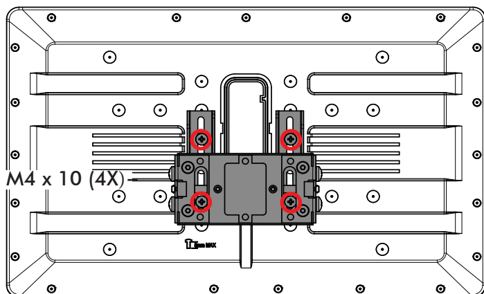
Display Bracket Right-side Up
