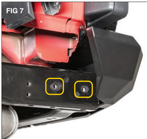
With assistance from another person, and with the tailgate partially open lift the bumper and gently slide it into the frame rails. Align the threaded holes with the holes in the frame rail. (FIG7)
