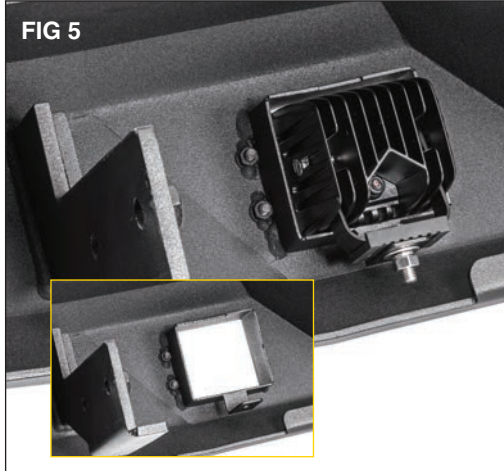
Pedestal Mounted Reverse Lamps: If installing pedestal mounted “Cube” style lamps, mount them as shown, using the 6mm Button Head bolts (B). (FIG 5)
