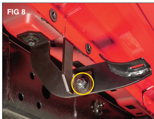
Next align the mounting slots between the two brackets and loosely install a 10mm bolt (A) with washers (G) on both sides and secure with a 10mm nylock nut (E) using a 16mm hex wrench and a 17mm socket. (FIG 8)
