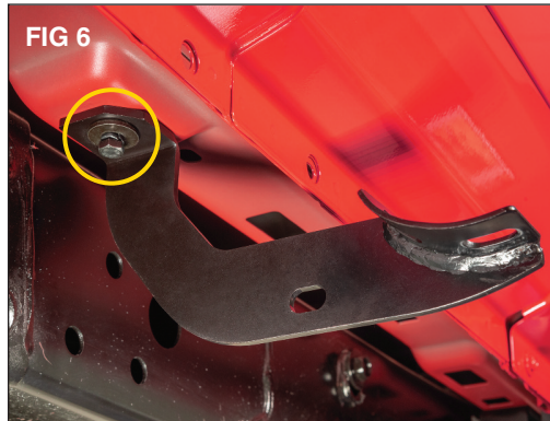
Align the hole in the step mounting bracket (PR) and loosely install using a 8 x 35mm bolt (B), lock washer (J) and flat washer (H). (FIG 6)
