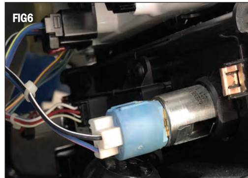
Gently pull the center panel away from the dash to release the clips and tilt it enough to access the 12 volt socket connection. Squeeze the white tab and dis-connect it. (FIG 6)
