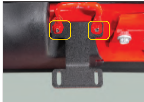
Re-install the footman loops and supplied light brackets using the original hardware. Bracket should be mounted under footman loop, as shown. (FIG 24)
