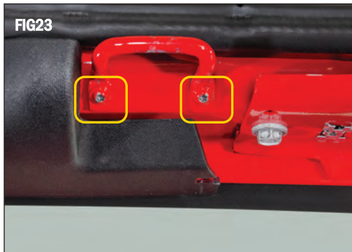
At the top of the windshield frame remove the screws holding in the footman loops using a T-25 torx driver. (FIG 23) Save the hardware.
