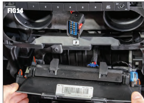
Lift the large dash top panel off and carefully set it aside. (highlighted in FIG13A)
