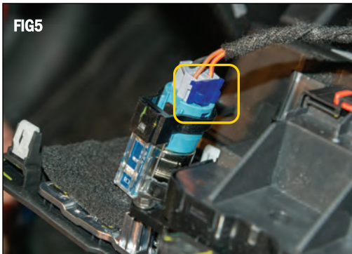
Tilt panel away enough to access the 12v socket connection. Squeeze the blue tab and disconnect it. (FIG 5)
