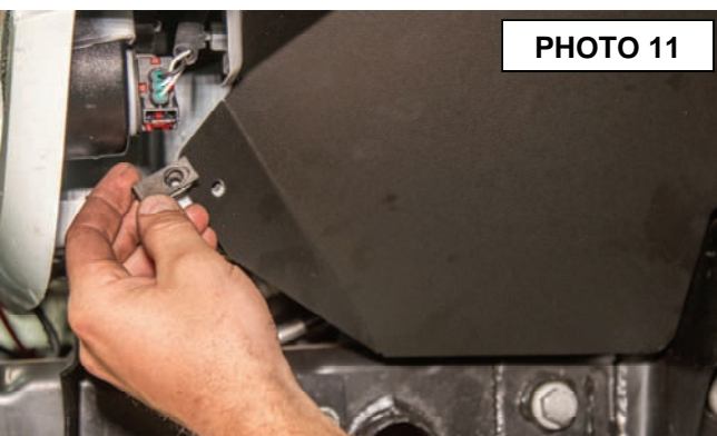
Install the 6mm clip nut.
