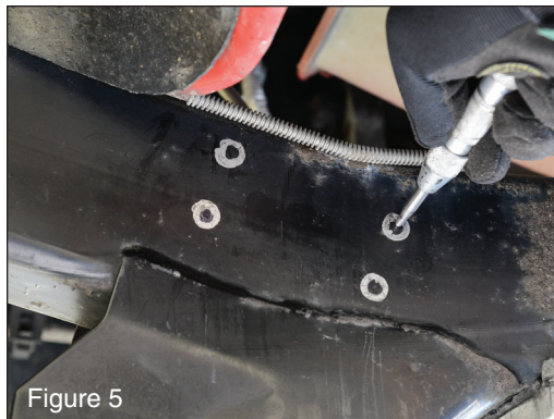
Figure 5 First, put your safety glasses on. Then using a center punch, mark the center of each of the holes. (Figure 5)
