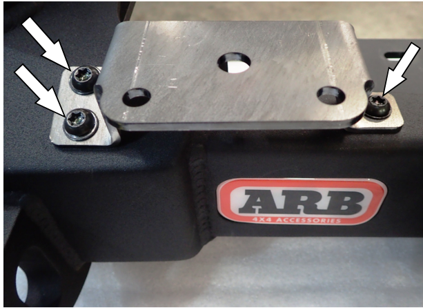
RH LIGHT BRKT SHOWN LH OPPOSITE
