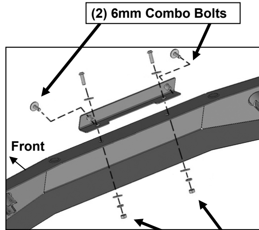
(Fig 8) License Plate Bracket attached to the Bull Bar
