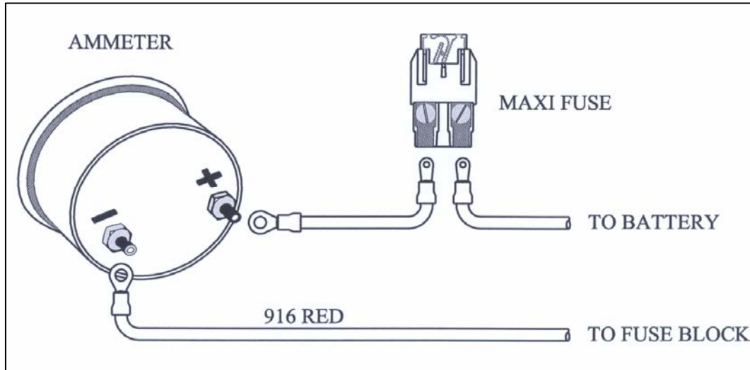
Figure 7.1 Ammeter & Maxi-Fuse
