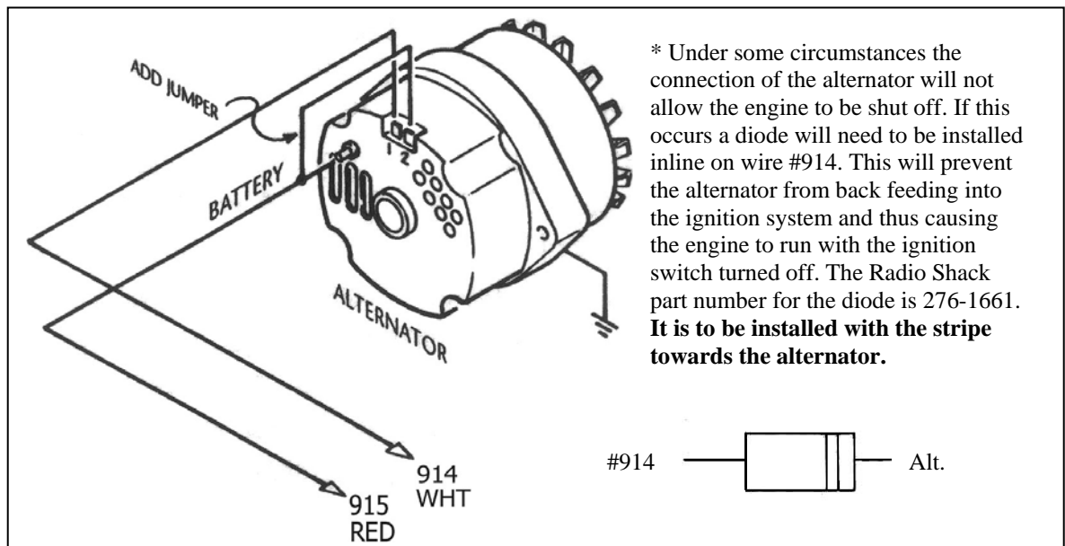
Figure 8.6 Delco Alternator (Internal Regulator)
