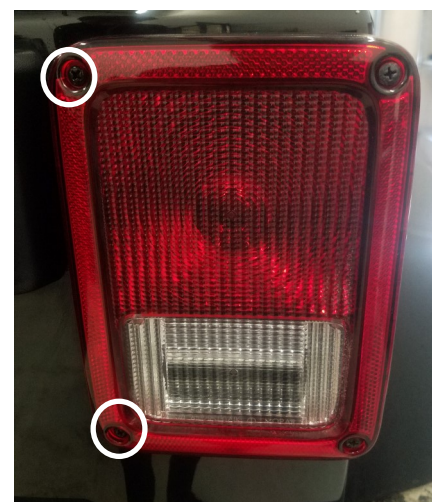
Figure 1: Remove 2 screws.
