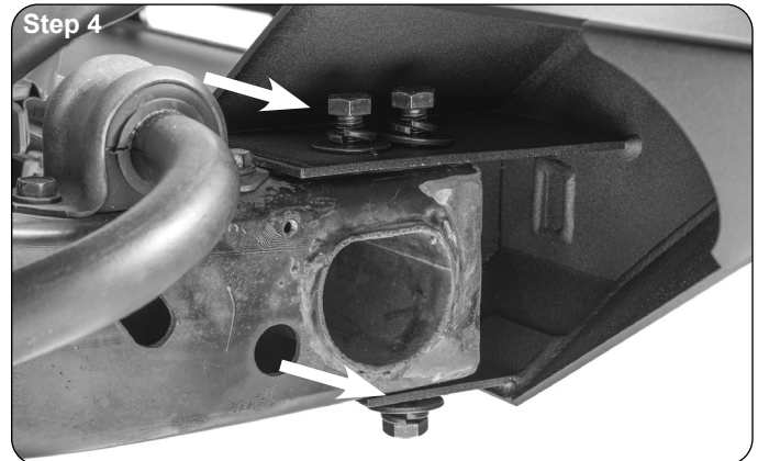
Bumper Installation: Install the new bumper over the frame rails and align the mounting holes. Install (6) 1/2" bolts, split washers, and flat washers into the upper and lower frame holes on the right and left side of the bumper. Tighten with a 3/4" wrench. (Step 4)
