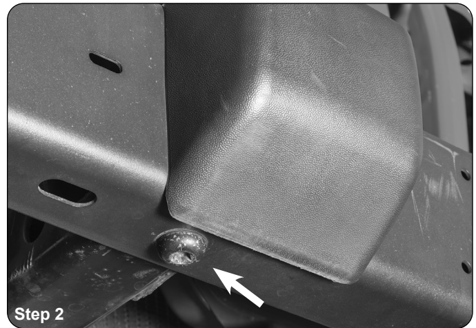
Remove the lower bumper bolts with and T55 socket on both sides. (Step 2) Remove and discard the factory bumper.
