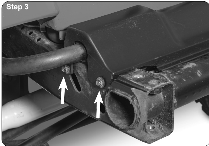
Remove the two 10mm bolts on either side of the Factory frame cover. Remove and discard the frame cover. (Step 3)
