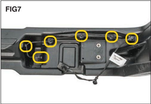
Remove the bumpers harness by gently prying on all tie wrap fasteners and disconnecting the license plate light. (FIG 7)
