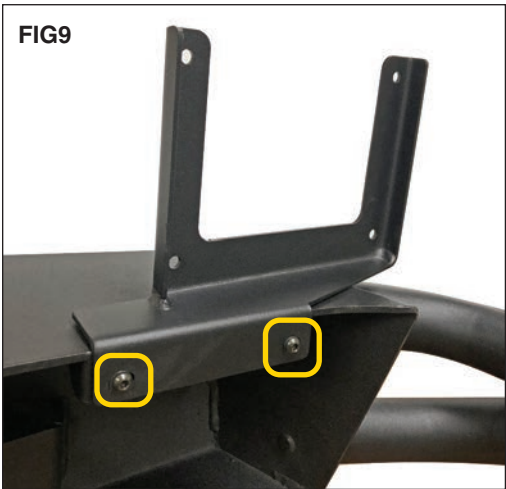
Install the license plate mount to the bumper using two M6 screws, two washers and two nuts. (FIG 9) The license plate will be installed with the remaining M6 hardware.
