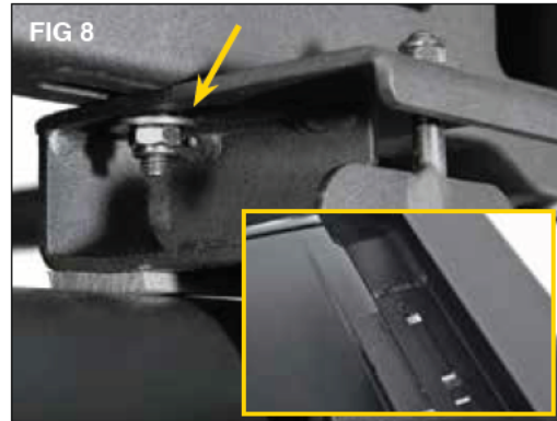
Loosely attach rack to brackets with the supplied M8 hex head bolts, washers and lock nuts. Each bolt will get two washers, one top and one bottom. (FIG 8)
