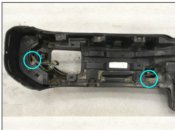
25. Disconnect 4 parking sensors connectors.
